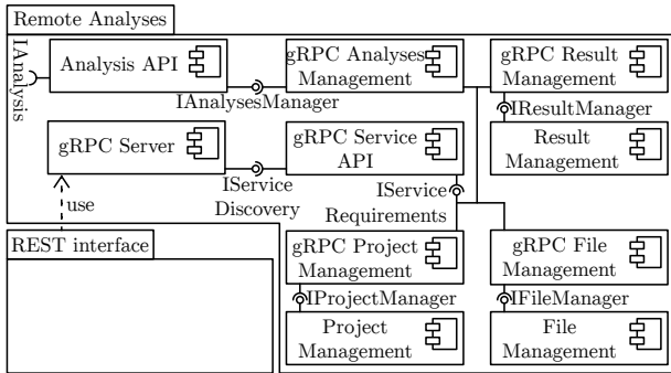
Figure 1: Remote Analysis Architecture (gRPC)
