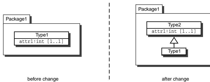
Figure 4: Example metamodel
