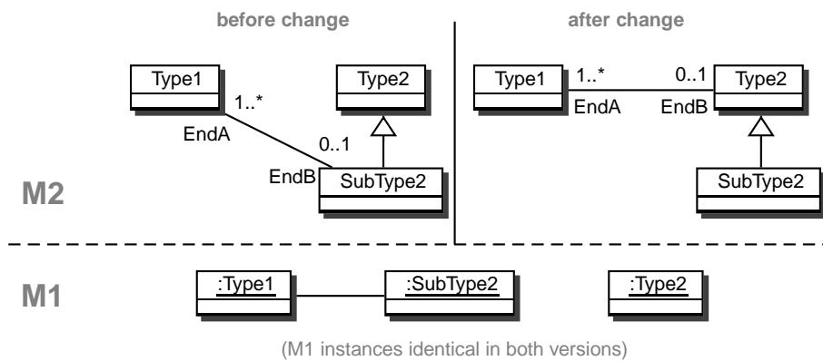
Figure 3: Example: Type change on an association end
