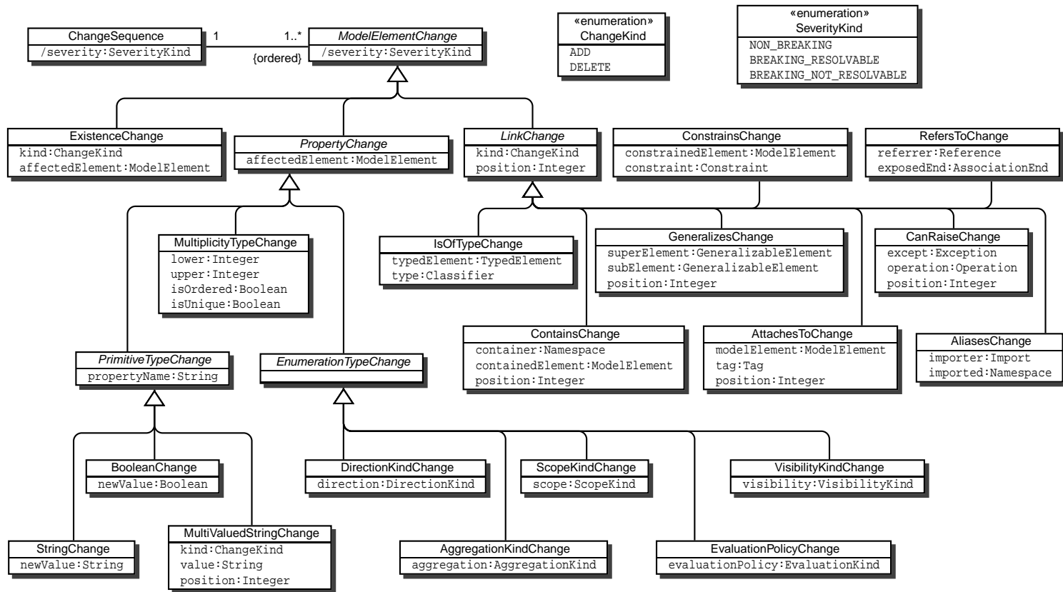
Figure 1: Change Metamodel
