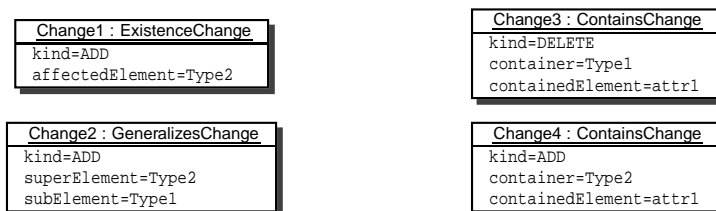
Figure 5: Change steps as Change Metamodel instances
