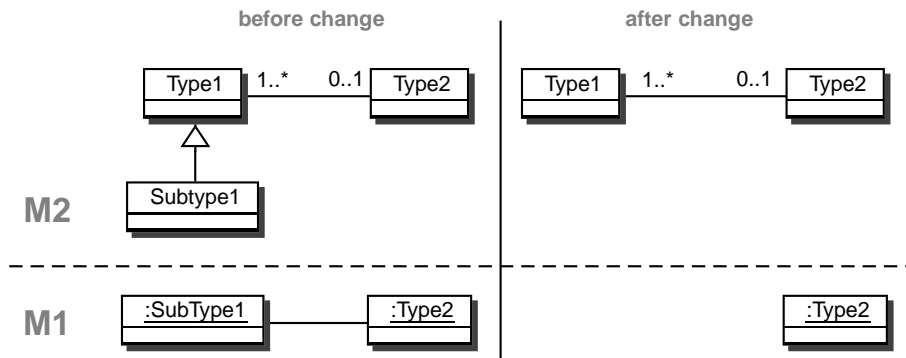
Figure 2: Example: Deletion of a class makes M1 data invalid
